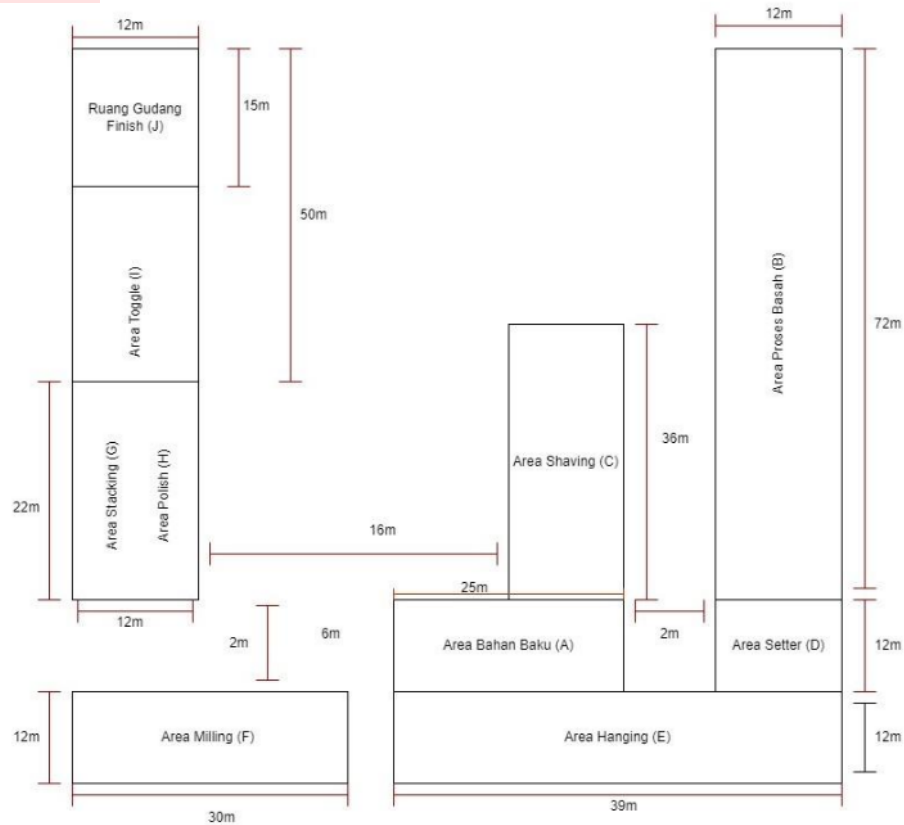
Gambar 3 Layout Usulan PT Adi Satria Abadi
