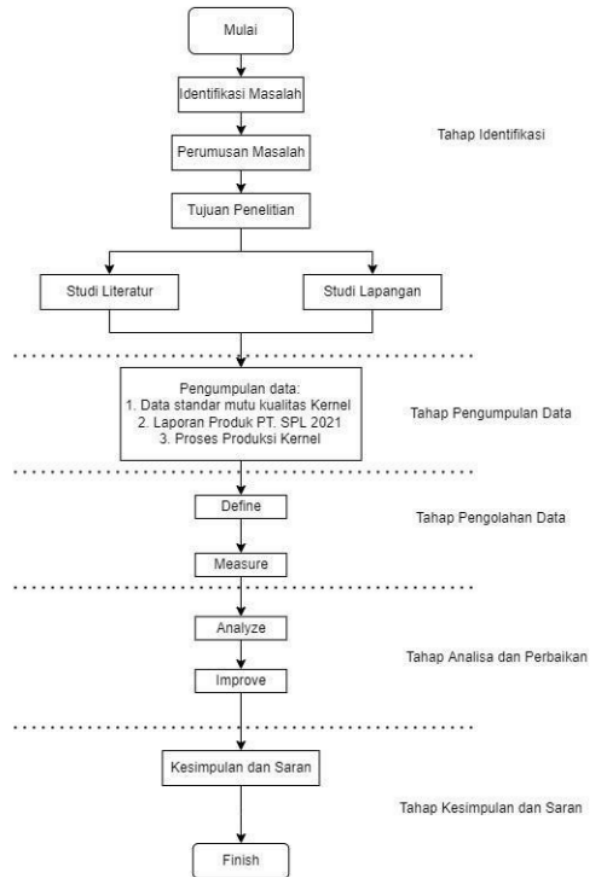
Gambar 1. Flowchart penelitian
