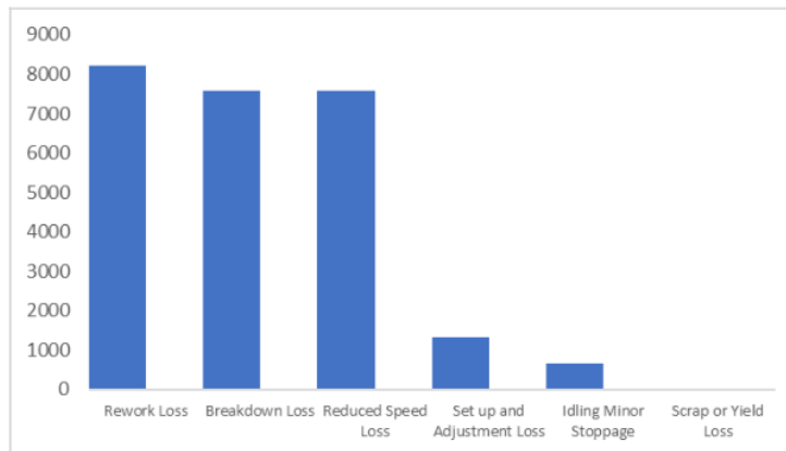
Gambar 1. Perbandingan losses
