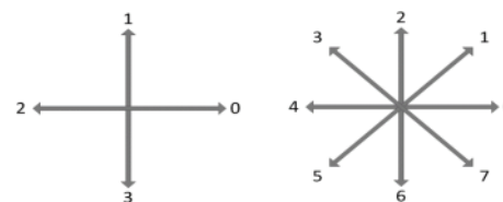
Figure 3: Chain Code (Freeman Code)
