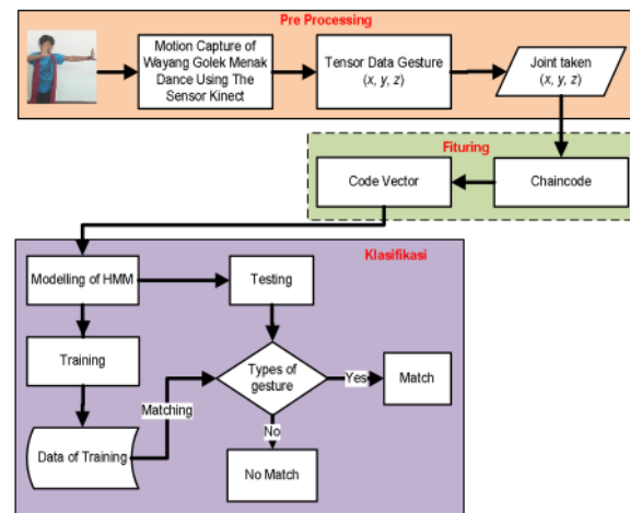
Figure 5: Flowchart recognition and classification Golek Menak dance
