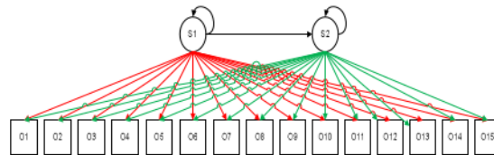
Figure 8: Architectural model HMM with 2 states and 15 observation
