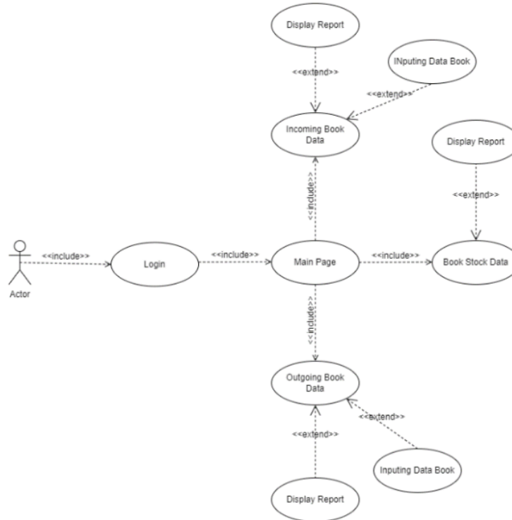
Fig. 4. Use case diagrams.
