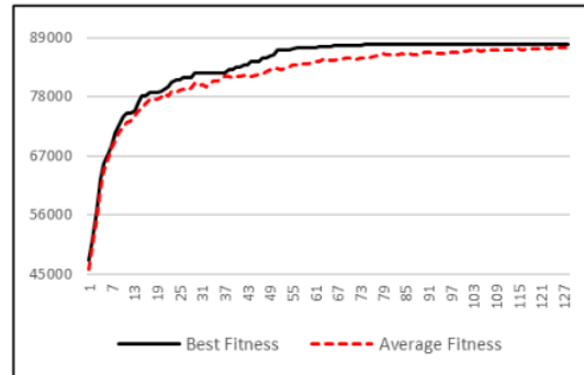
Fig. 4. The evolution process shows that every generation has high quality chromosome that has fitness value close to the best one.
