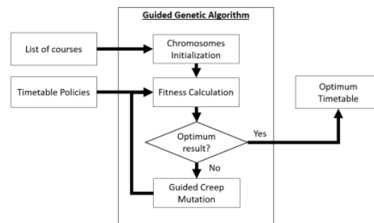
Fig. 1. The system architecture that is developed in this research.
