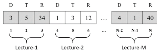
Fig. 2. Design of chromosome that has N genes that consist of M courses. Each course schedule is encoded with 3 chromosomes that represents the Day (D), Time (T), and Room (R).
