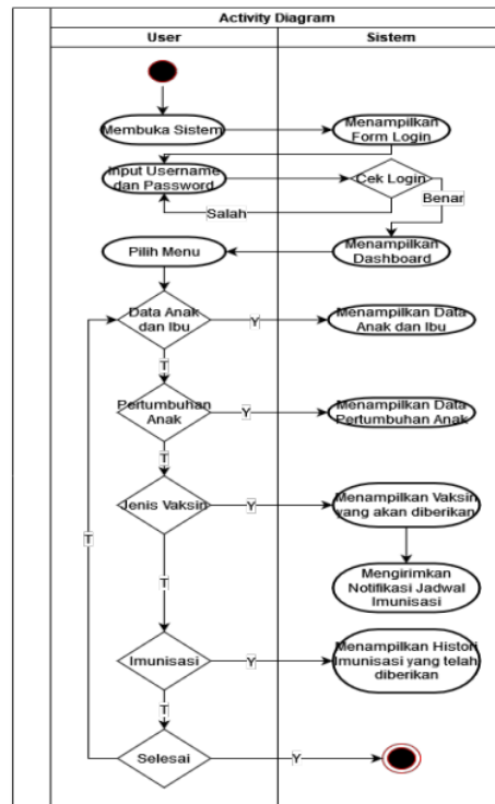
Gambar 3. Activity user
