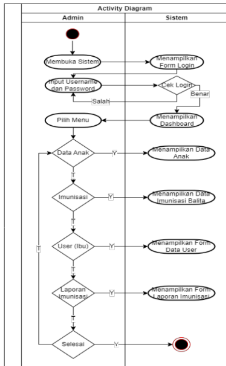
Gambar 2. Activity admin
