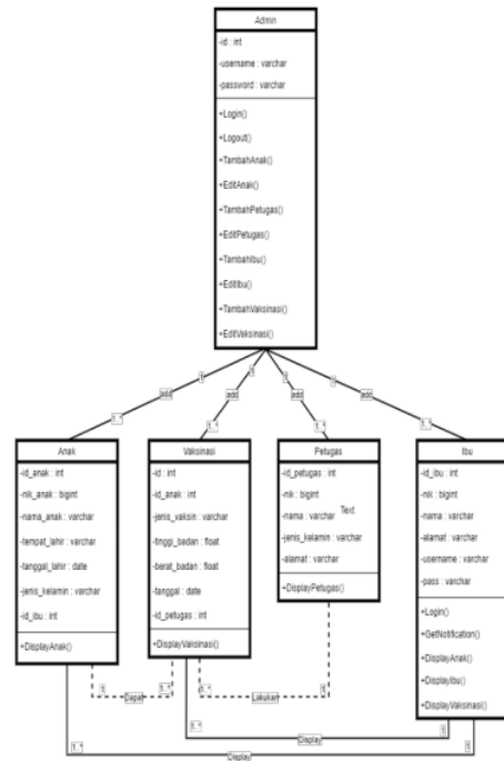
Gambar 5. Class diagram
