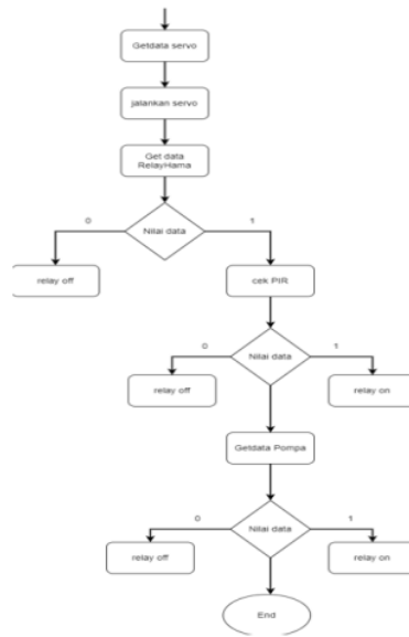
Gambar 8 (c). Flowchart ESP8266 (lanjutan)
