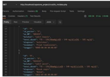
Gambar 6. Input Database
