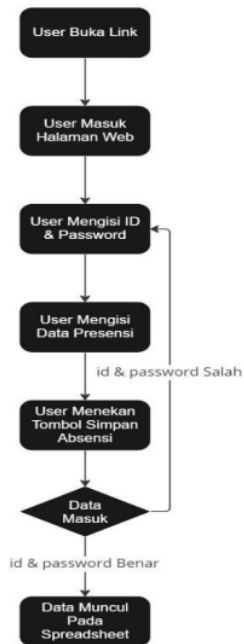
Gambar 2. Flowchart Sistem
