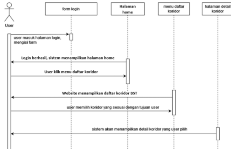
Gambar 1. Sequence Diagram
