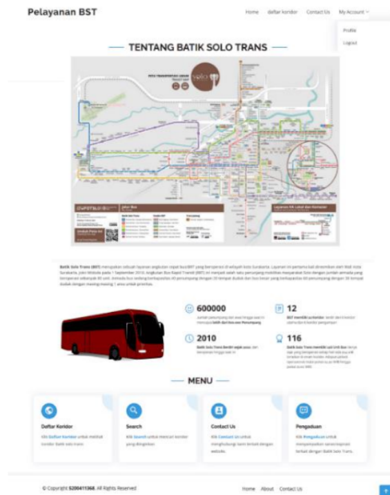
Gambar 4. Home Page
