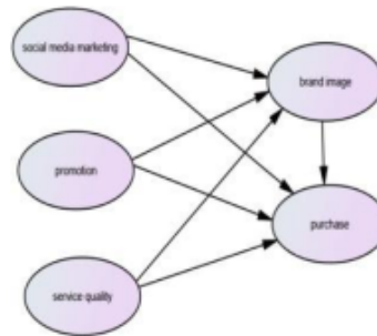
Fig. 1. Research Model
