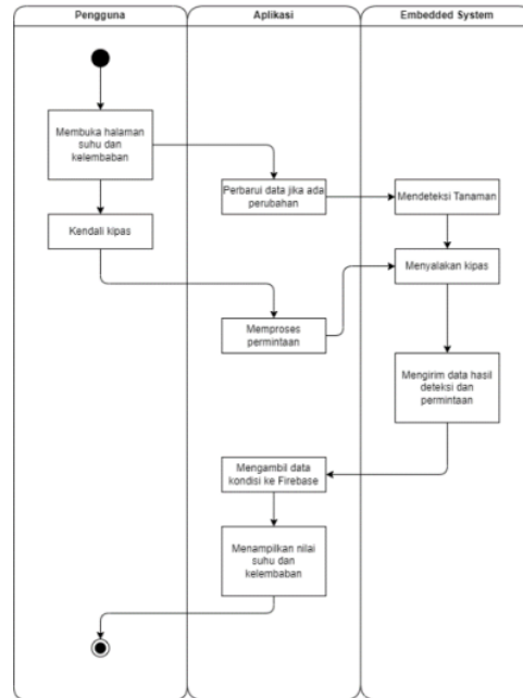
Gambar 2. Diagram Activity Aplikasi Monitoring
