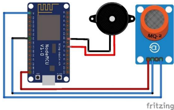
Gambar. 2 Rangkaian Hardware
