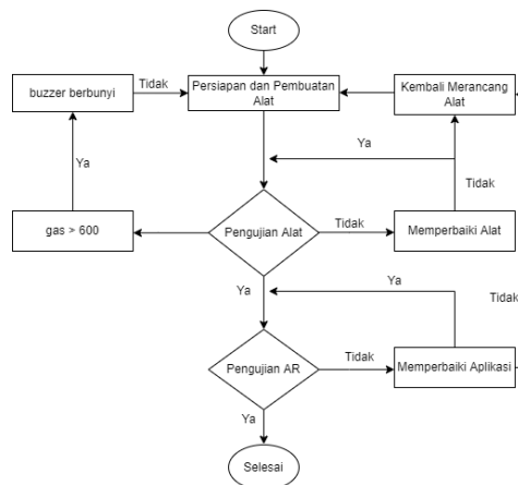
Gambar.1 Flowchart Sistem
